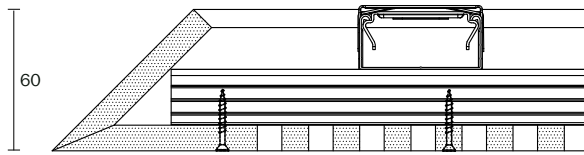
Plasterboard ceiling sails with bevelled upstand
